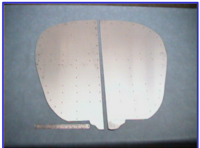
Firewall Left & Right
