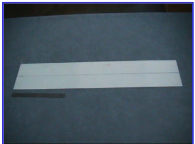
Aileron Premould Strip 95 x 1000mm
